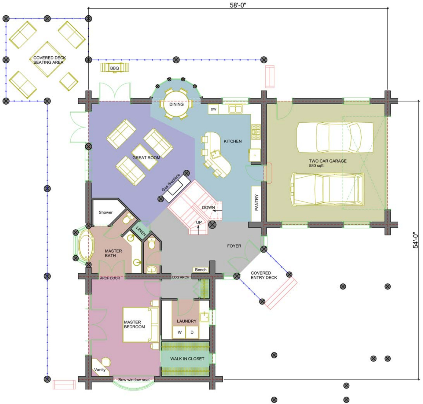
FIRST FLOOR PLAN AREA: 1700 SQ.FT.
