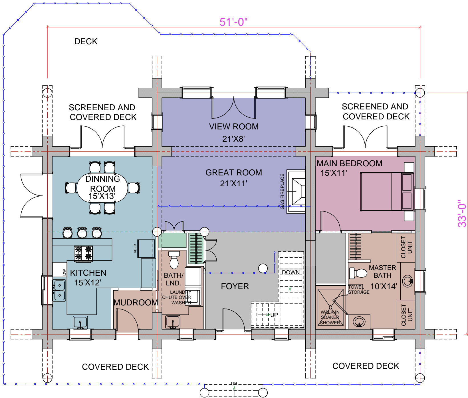
FIRST FLOOR PLAN AREA: 1485 SQ.FT.
