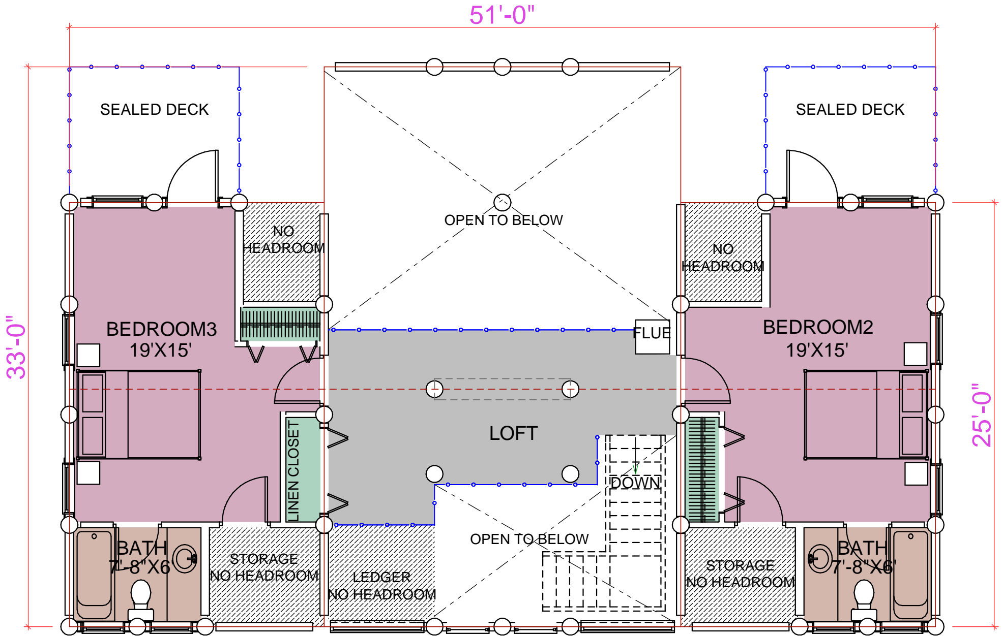
SECOND FLOOR PLAN AREA: 819 SQ. FT.
