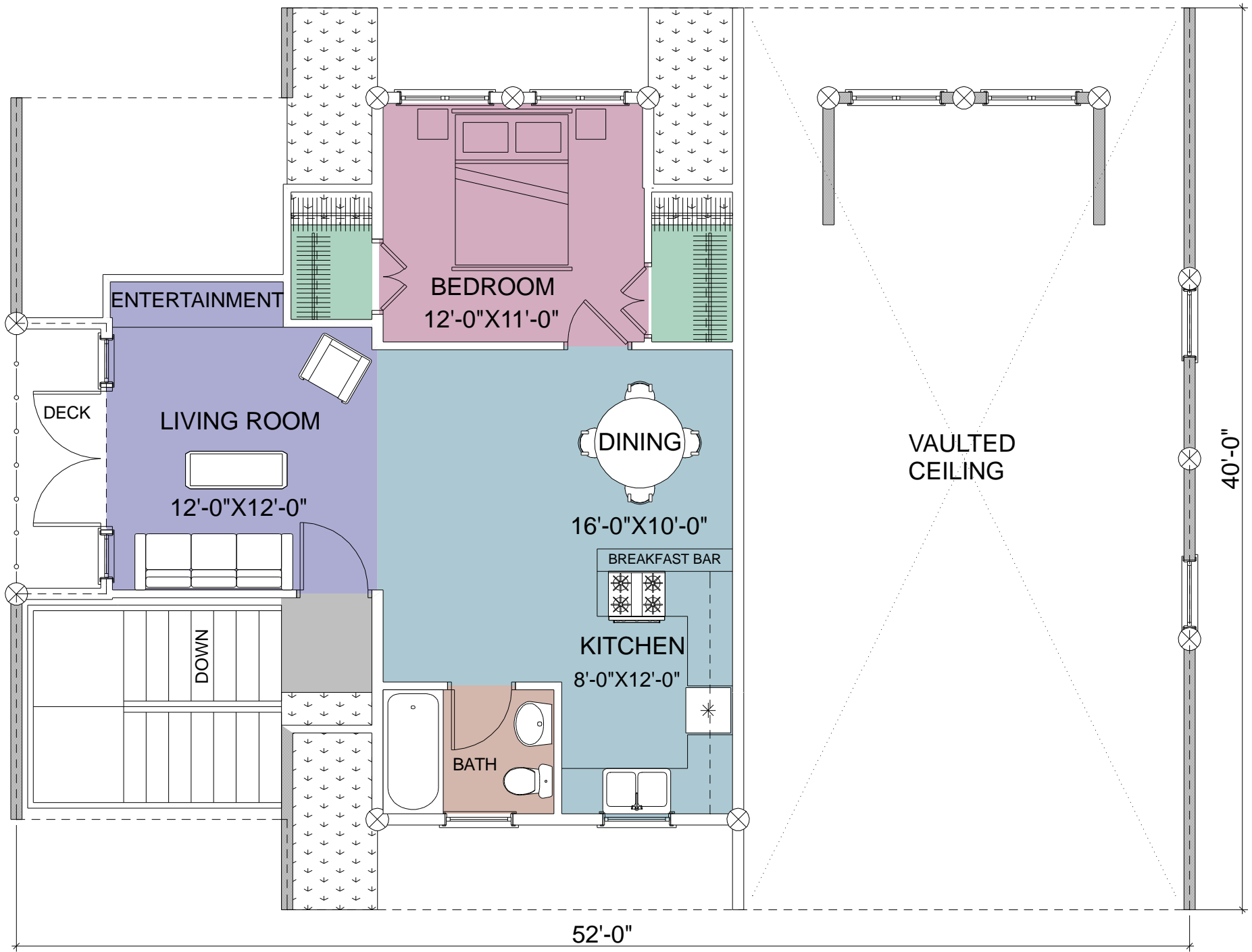
SECOND FLOOR PLAN AREA: 681 SQ. FT.
