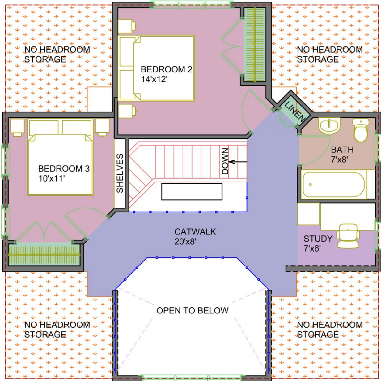
SECOND FLOOR PLAN AREA: 610 SQ. FT.
