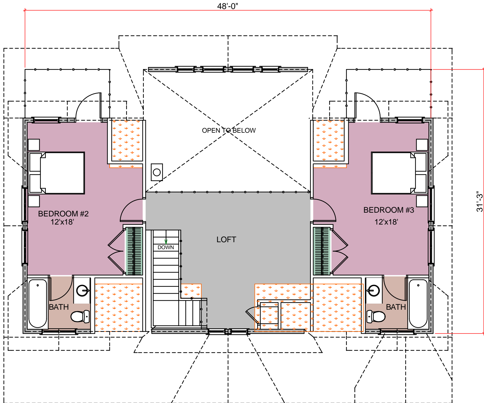
SECOND FLOOR PLAN AREA: 842 SQ. FT.
