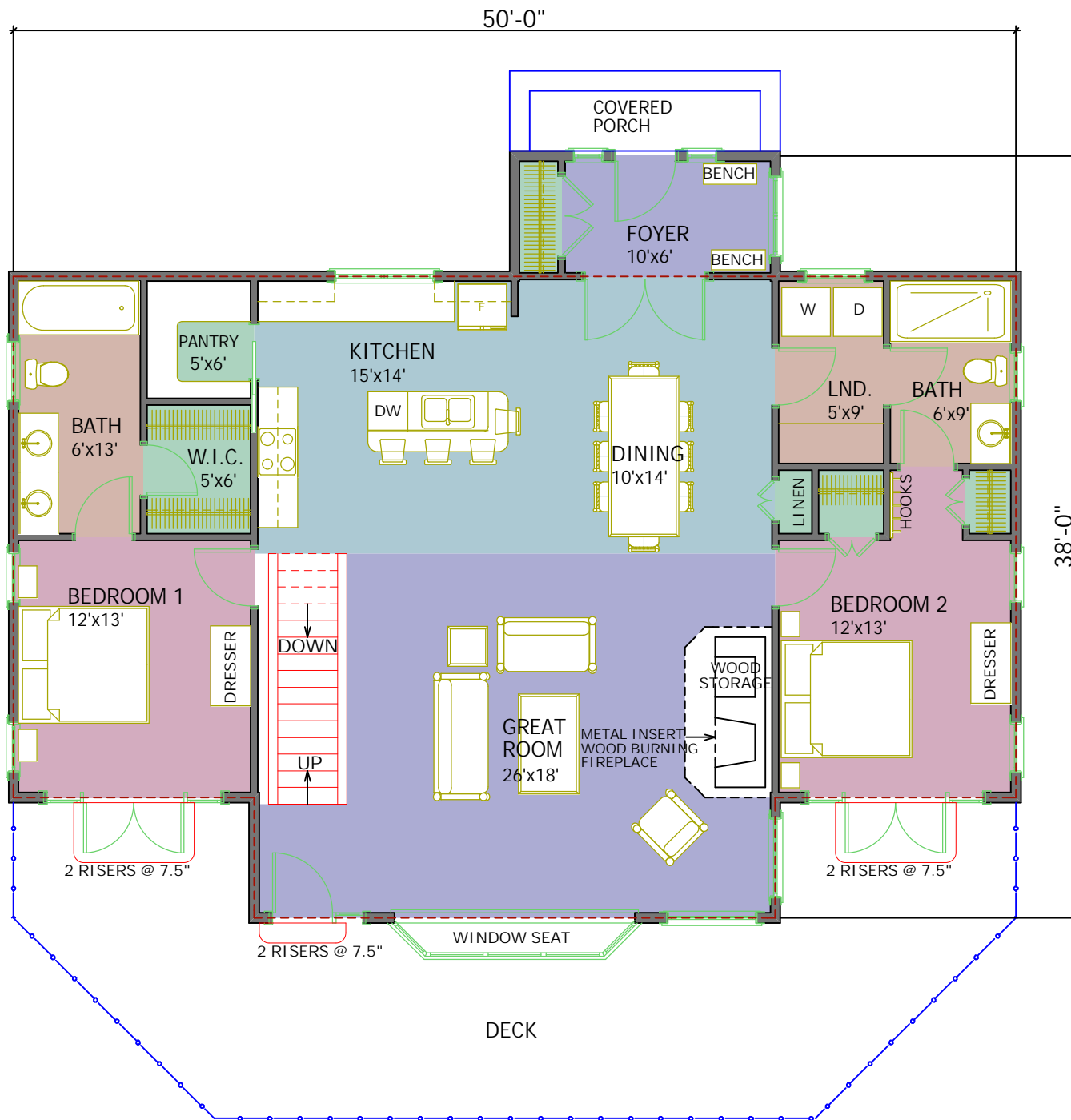
FIRST FLOOR PLAN AREA: 1578 SQ.FT.
