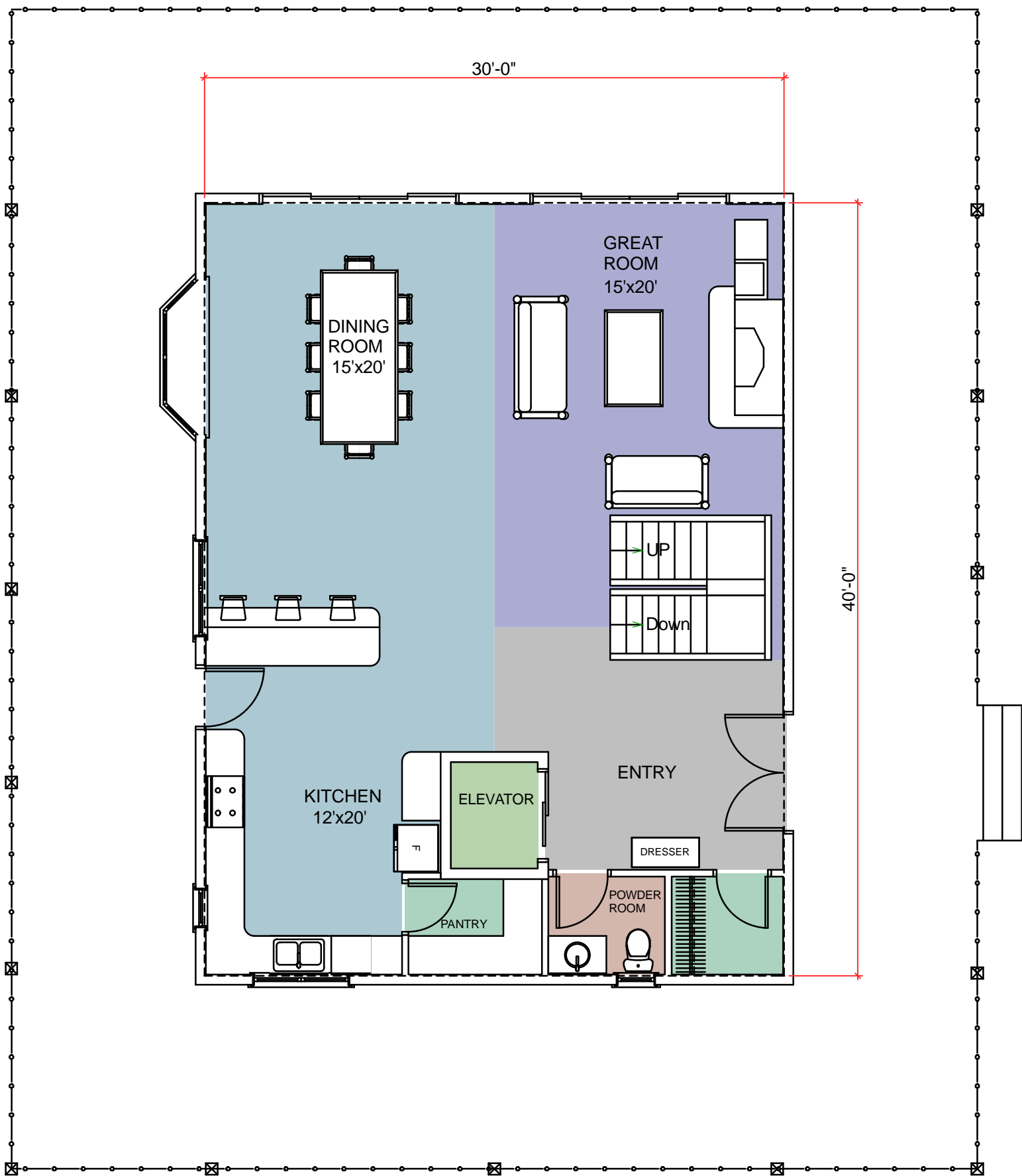
FIRST FLOOR PLAN AREA: 1470 SQ.FT.
