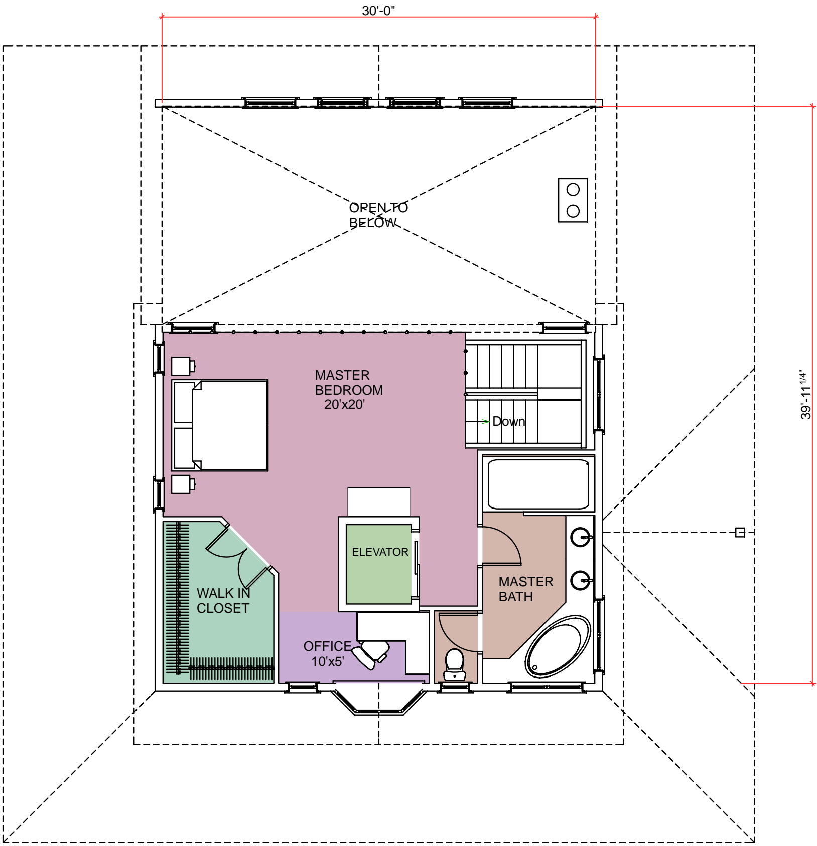
SECOND FLOOR PLAN AREA: 654 SQ. FT.
