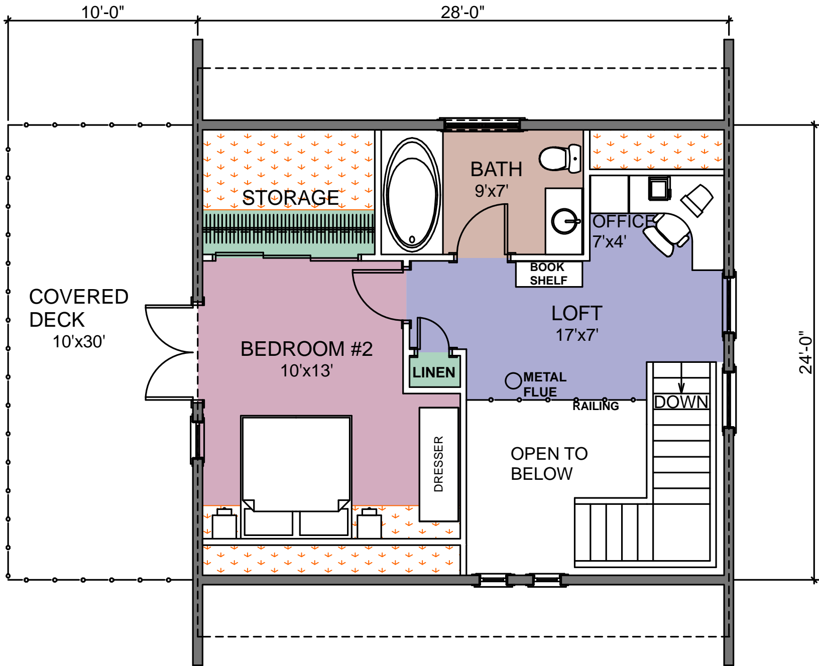
SECOND FLOOR PLAN AREA: 411 SQ. FT.
