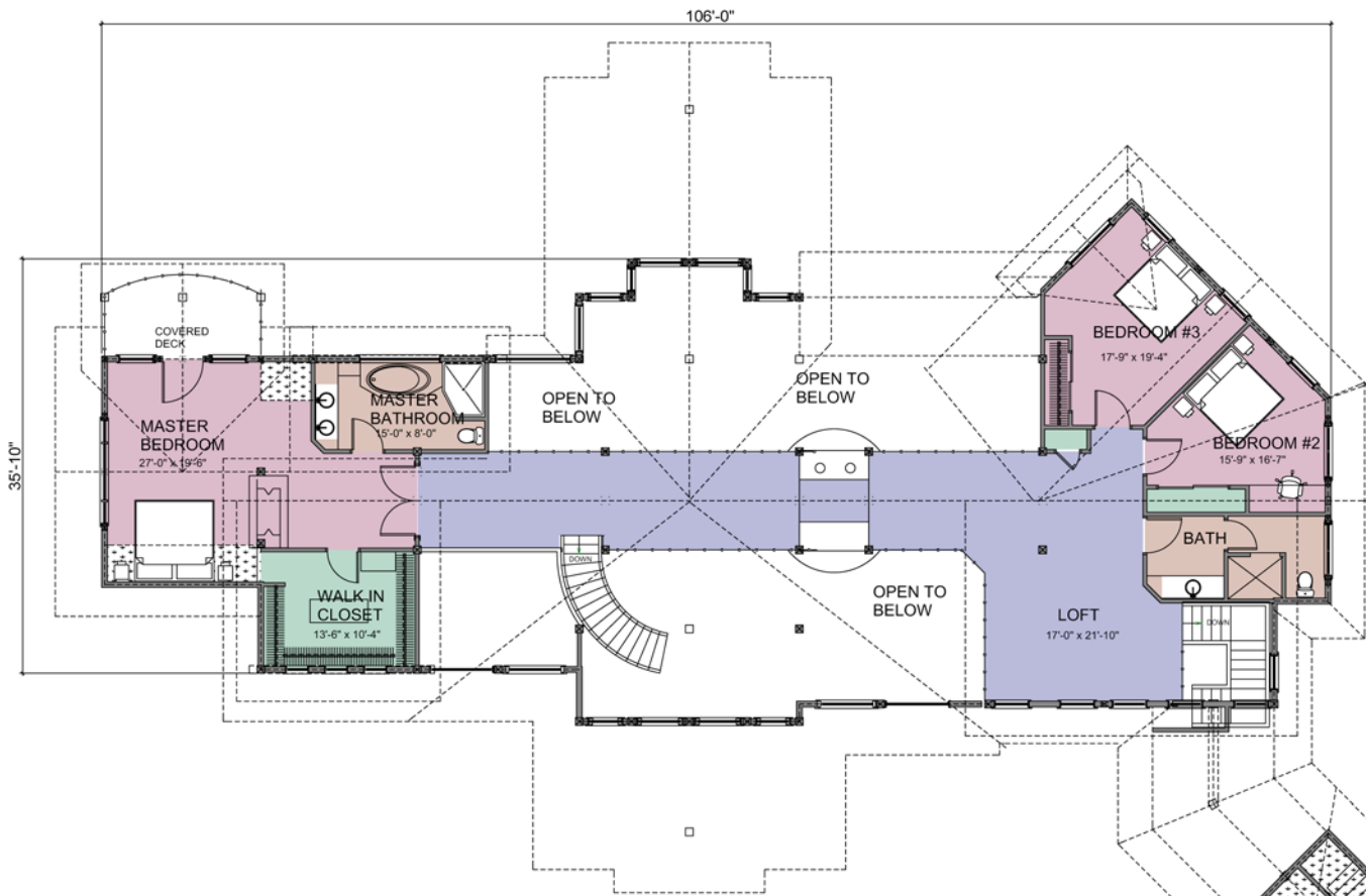
SECOND FLOOR PLAN AREA: 1954 SQ. FT.
