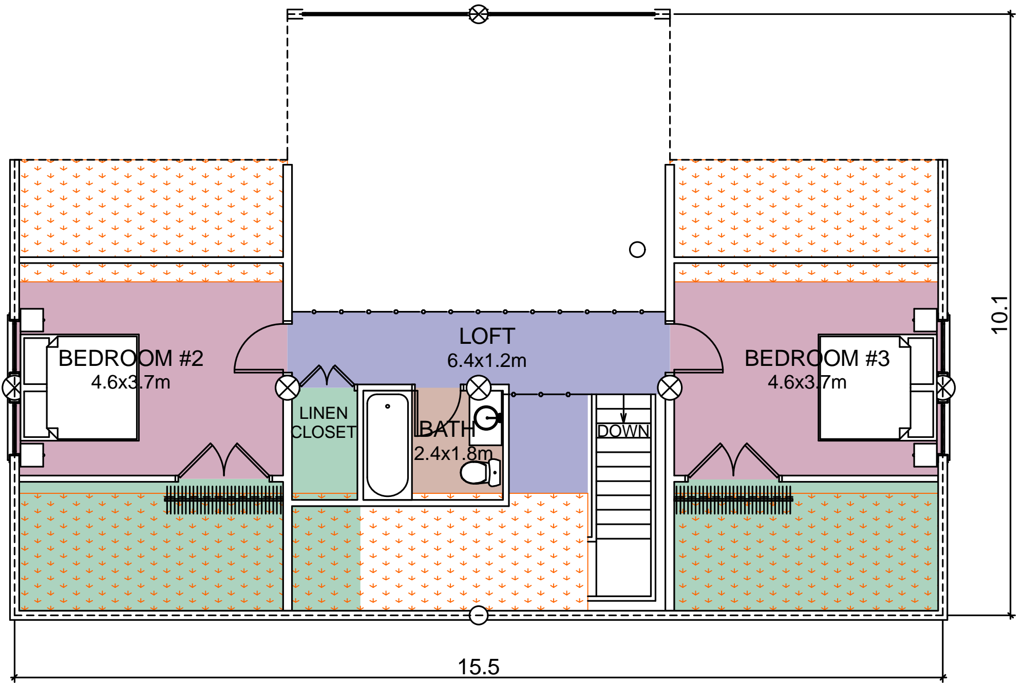
SECOND FLOOR PLAN AREA: 69 m 2
