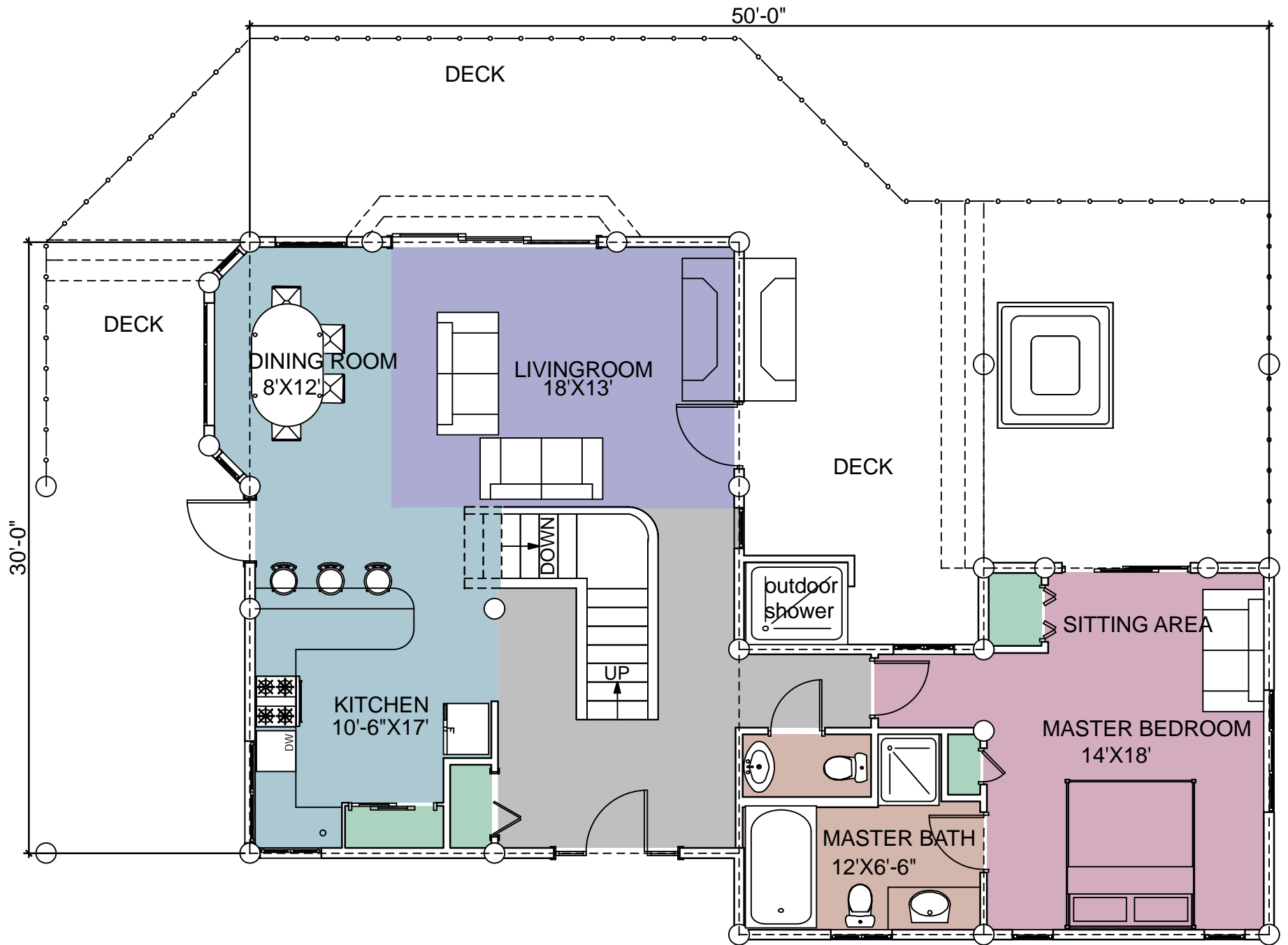
FIRST FLOOR PLAN AREA: 1198 SQ.FT.
