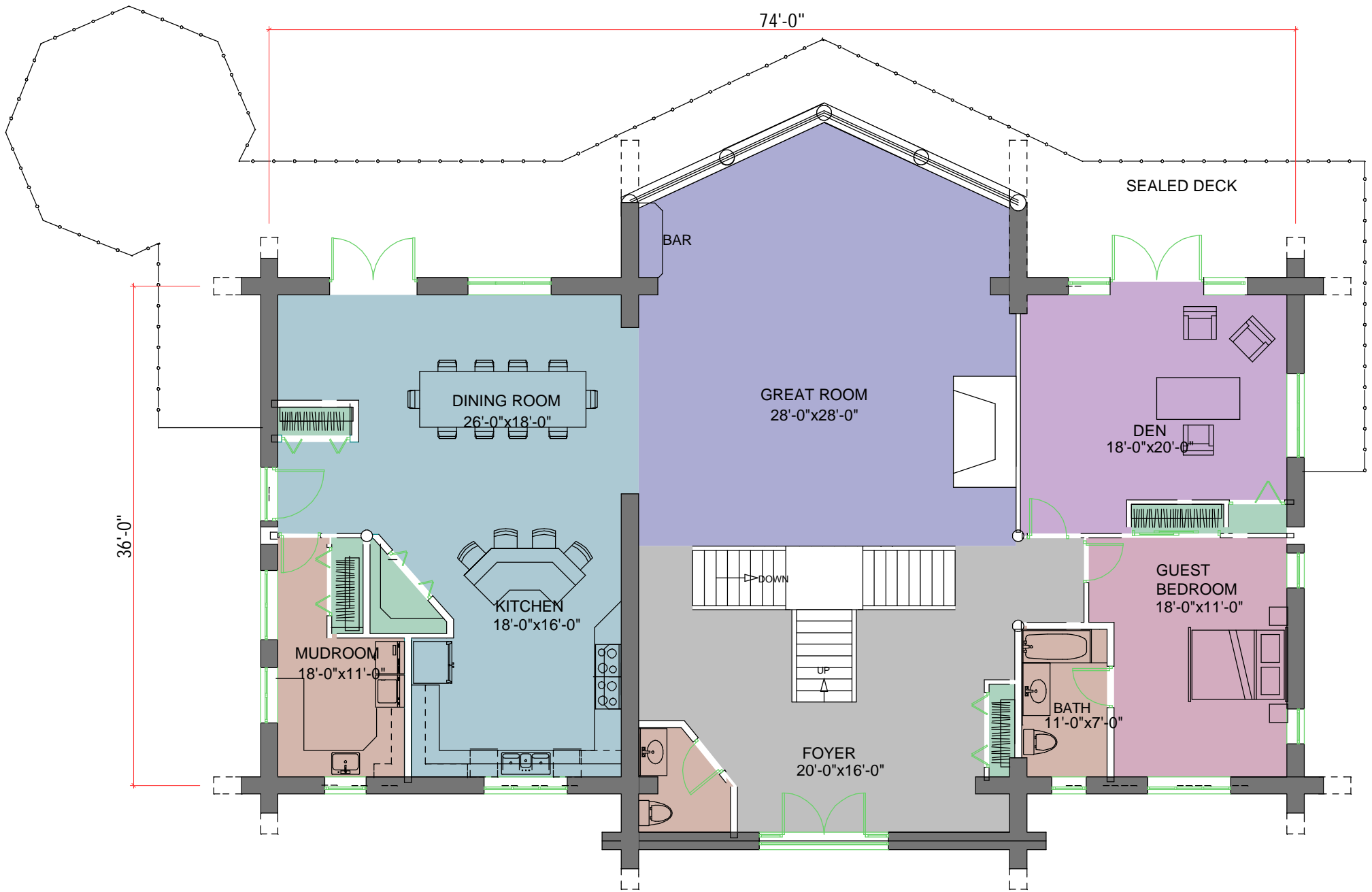
MAIN FLOOR PLAN AREA : 3100 SQ.FT.
