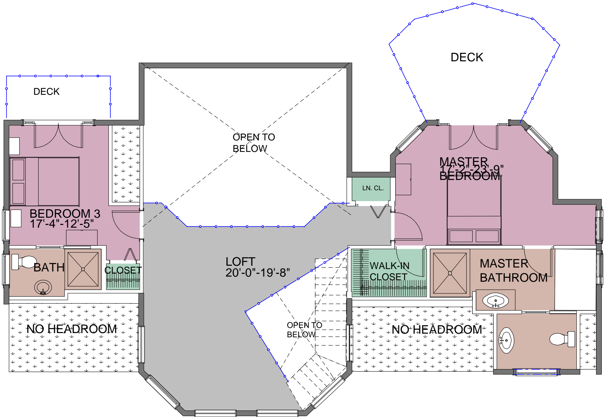
SECOND FLOOR PLAN AREA: 886 SQ. FT.
