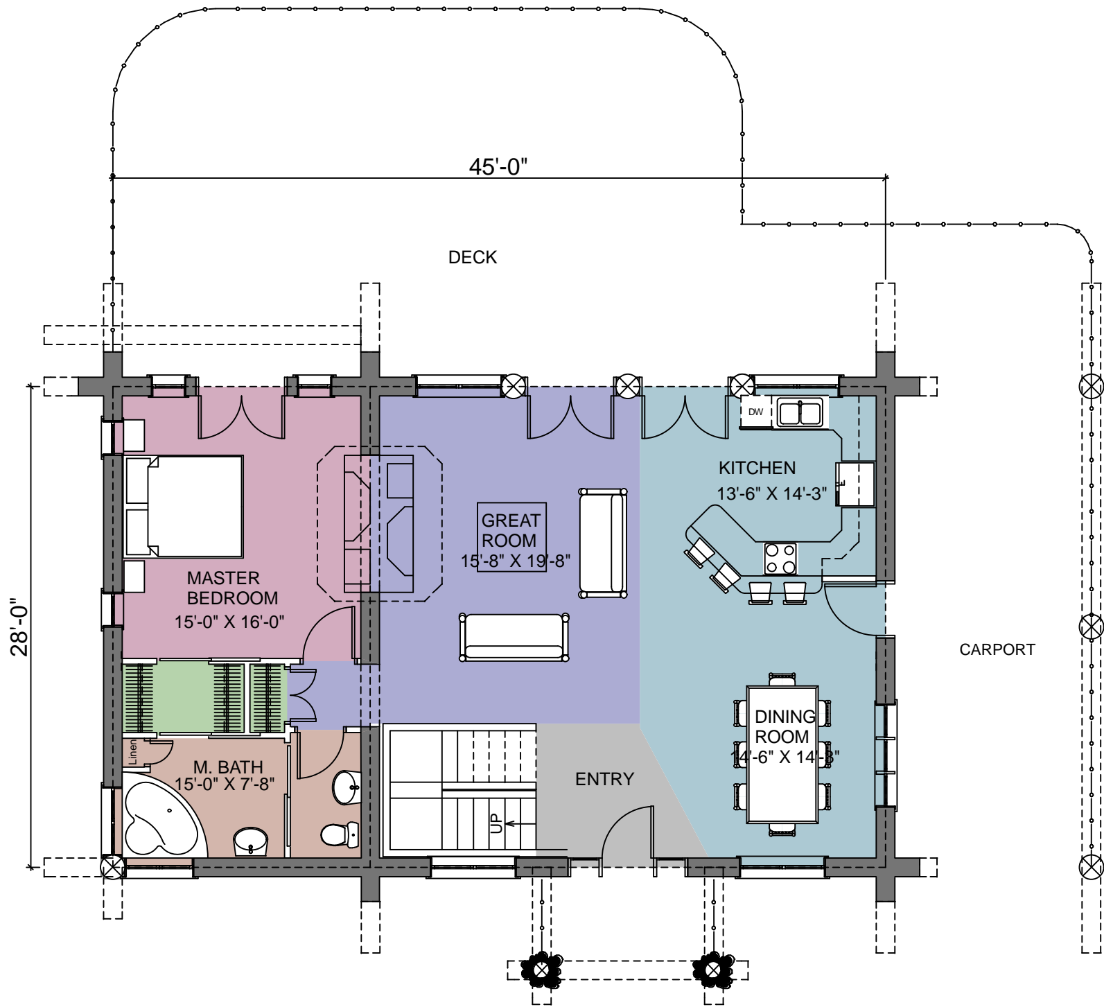
FIRST FLOOR PLAN AREA: 1297 SQ.FT.
