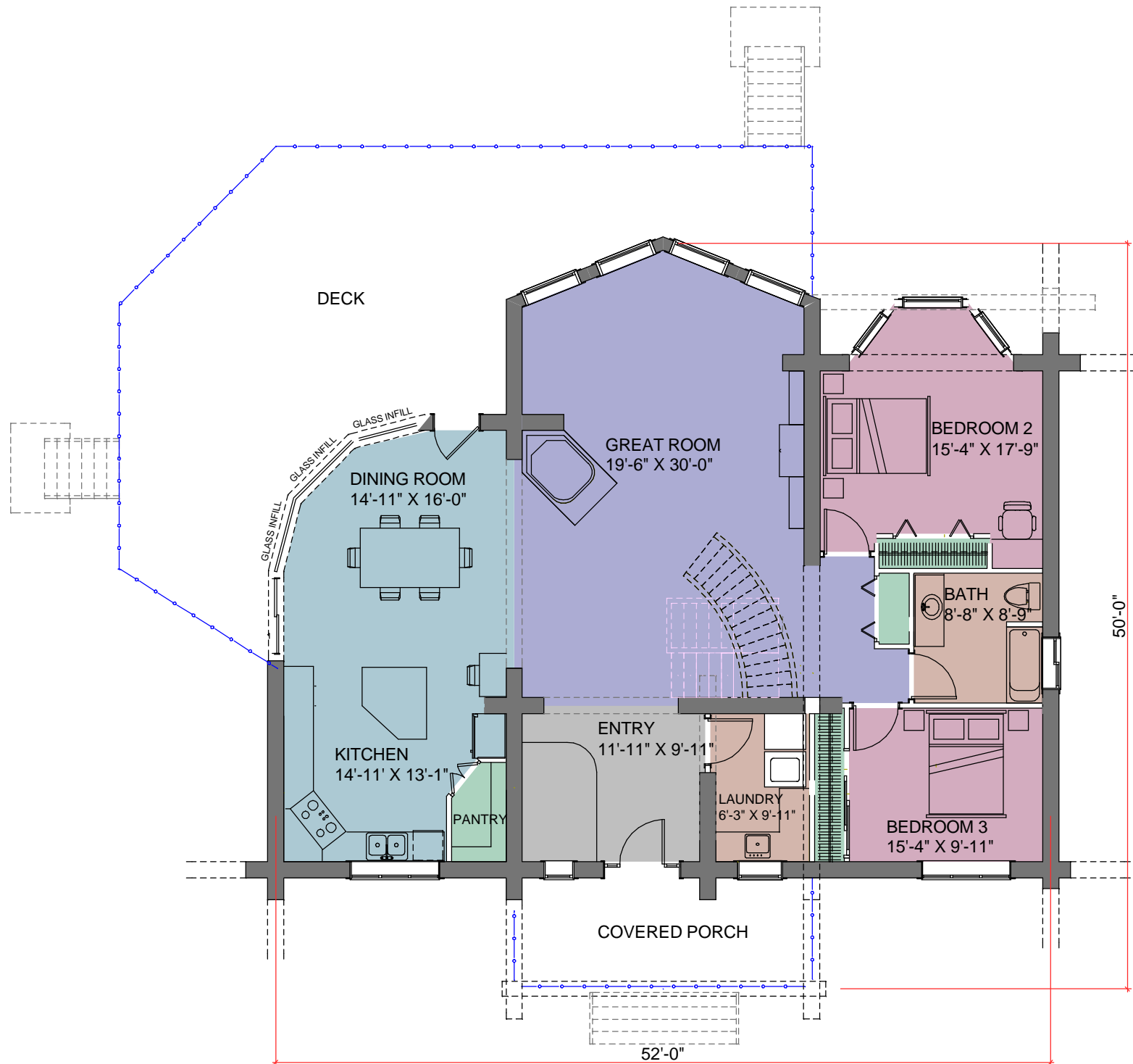
FIRST FLOOR PLAN AREA : 1,877 SQ.
