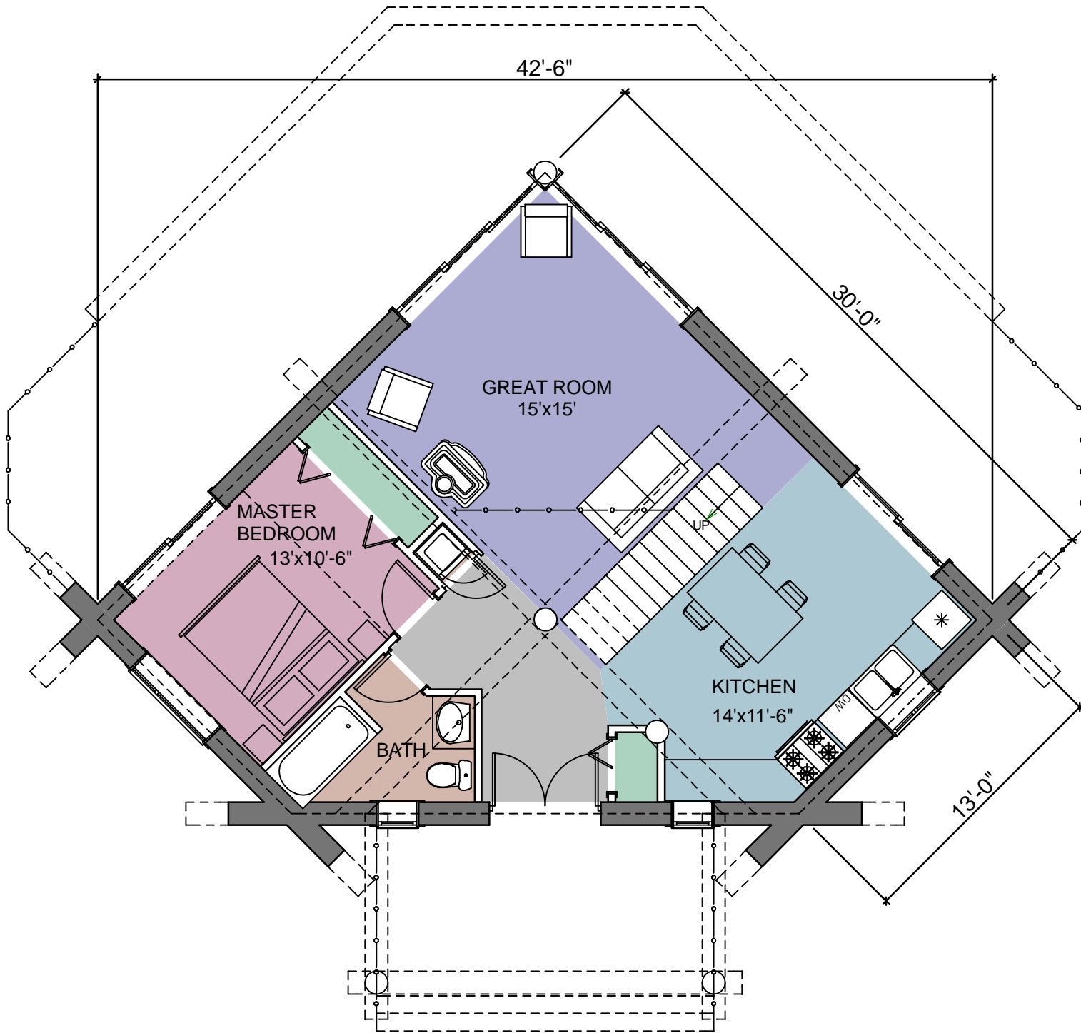
FIRST FLOOR PLAN AREA: 782 SQ. FT.
